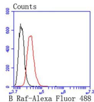
Fig. 2. Flow cytometric analysis of HeLa cells with B Raf antibody at 1/50 dilution (red) compared with an unlabelled control (cells without incubation with primary antibody; black). Alexa Fluor 488-conjugated goat anti rabbit IgG was used as the secondary antibody.
